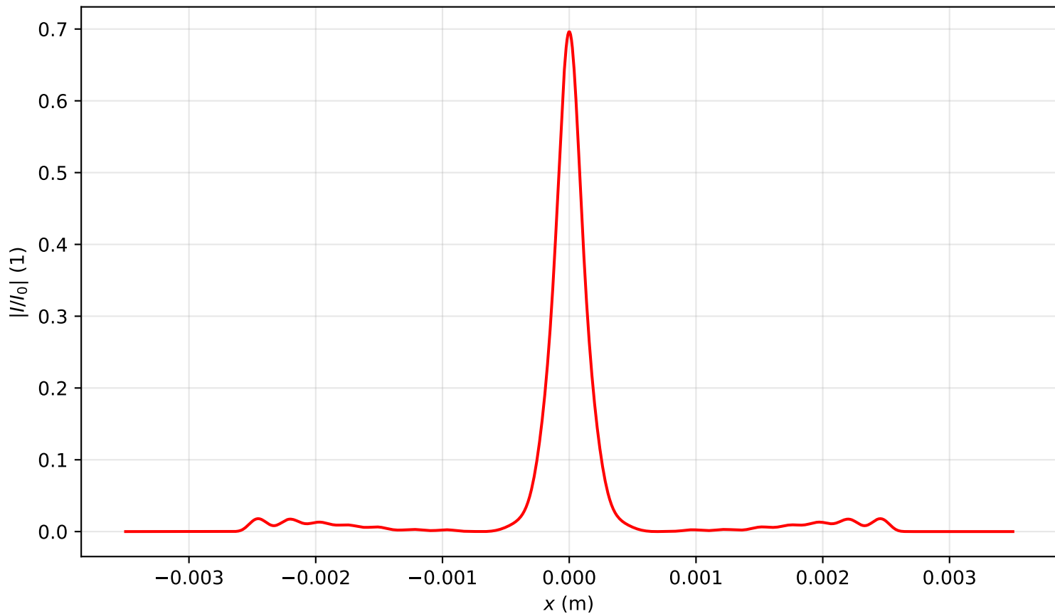
Intensity profile I(x, y = 0, z = 1.751)/I_0 , P_{in}=7.0P_{cr} , artificial time
